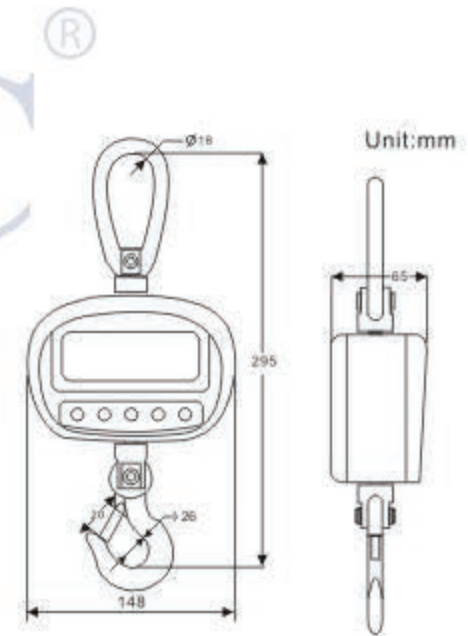
Dimensioned Drawing for GSE
